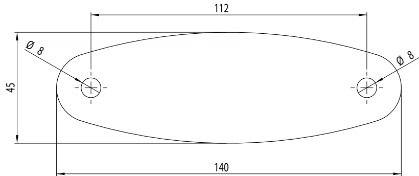
Desktop Mount Hole Dimensions
